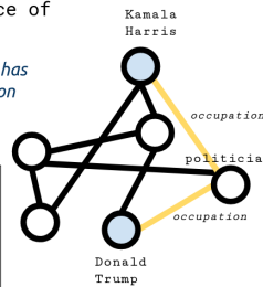
Figure 2: Illustration of our proposed path-based knowledge infusion method.
