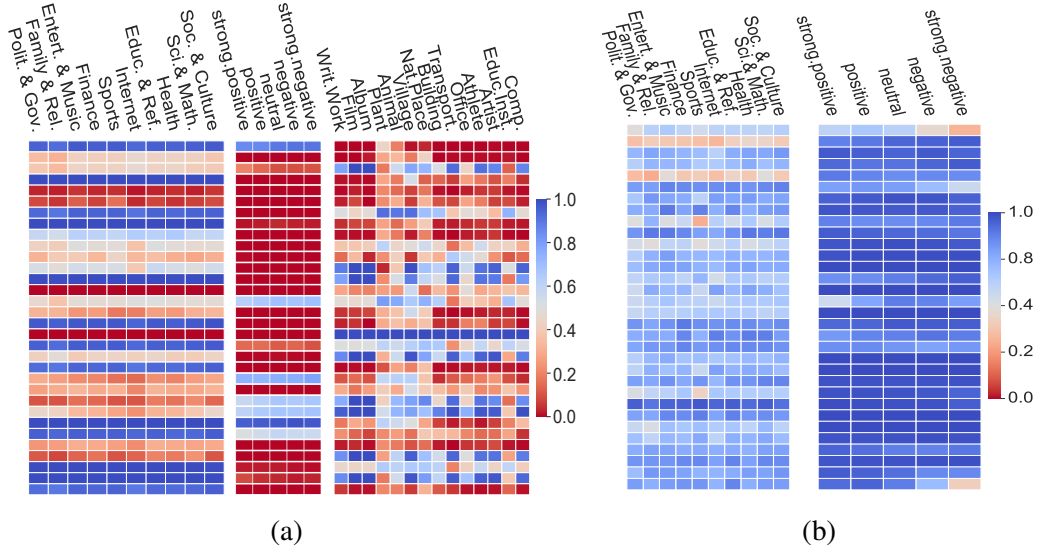
Fig. 6.4 Heat maps of \gamma_{class} (Section section 6.3.4). (a) \gamma_{class} of 32D - from left to right: Yahoo, Yelp, DBpedia. (b) contiguous 32D out of 768D of \gamma_{class} - from left to right: Yahoo, Yelp.
